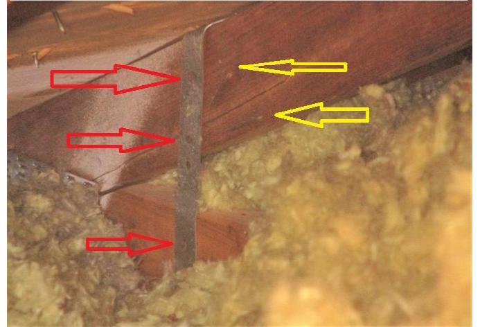
#4) roof to wall attachment: single wrap- front view
