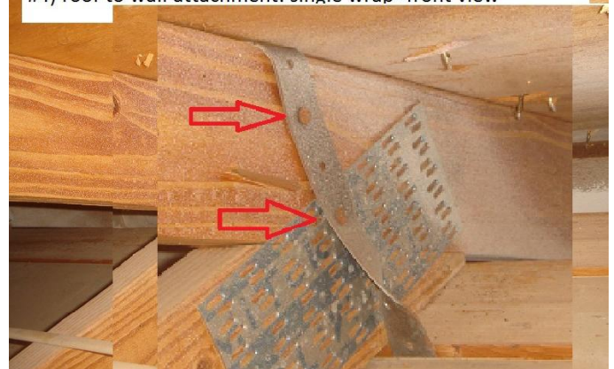
#4) roof to wall attachment: single wrap- front view
